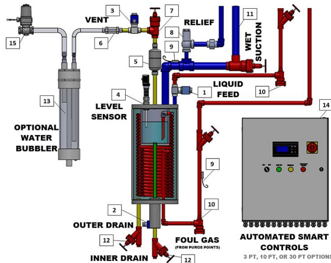
Figure 1: PUR Air Purger General Layout
