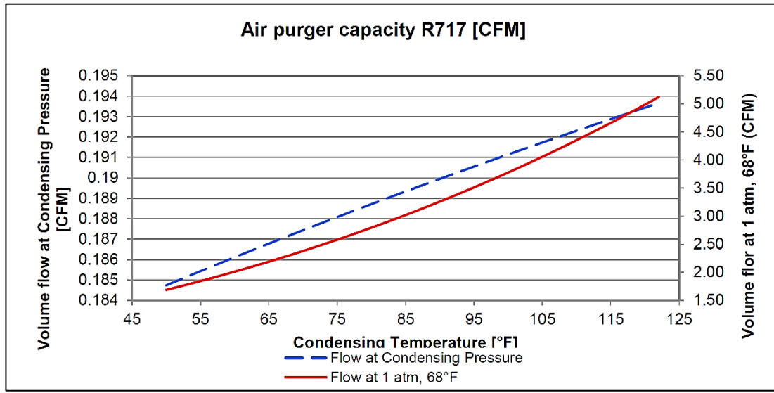
Figure 2: Purger Capacity
