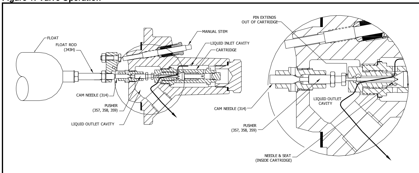
Figure 1: Valve Operation
