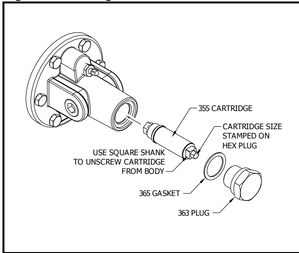
Figure 5: Cartridge Removal
