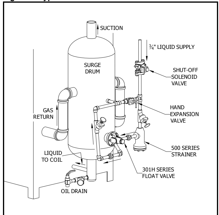
Figure 3: Typical Installation
