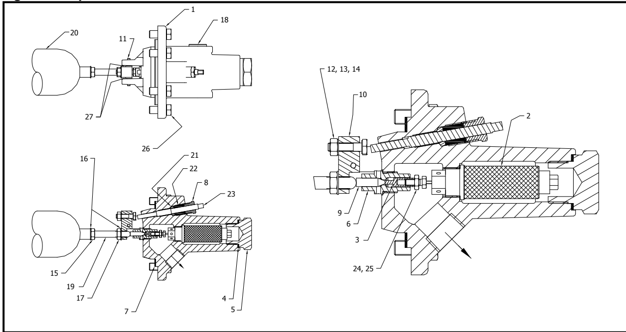
Figure 4: Replacement Parts
