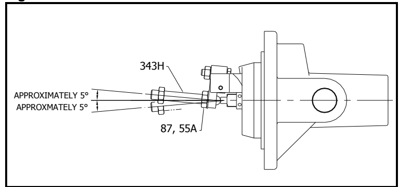
Figure 7: Rod Movement
