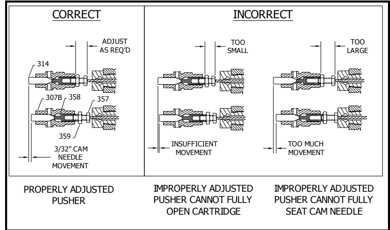
Figure 7: Rod Movement
