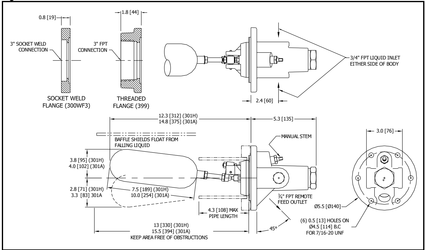
Figure 2: Dimensions
