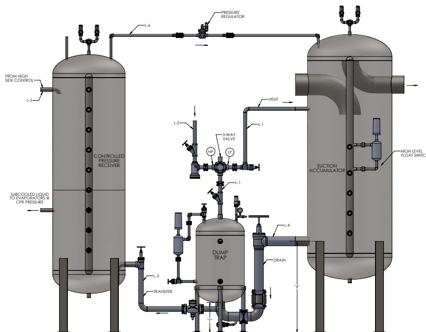
Typical GDRS System Layout (Vertical Dump Trap shown)
