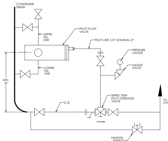
Typical High Side Control Schematic
