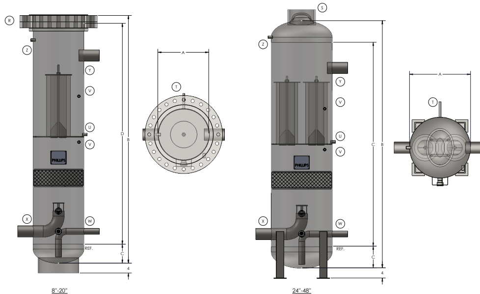
COALESCENT OIL SEPARATOR DIMENSIONS
