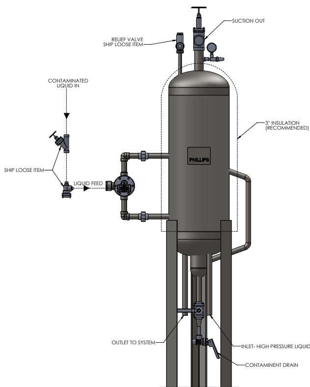
ANH-CV-A TRIM LEVEL SHOWN
