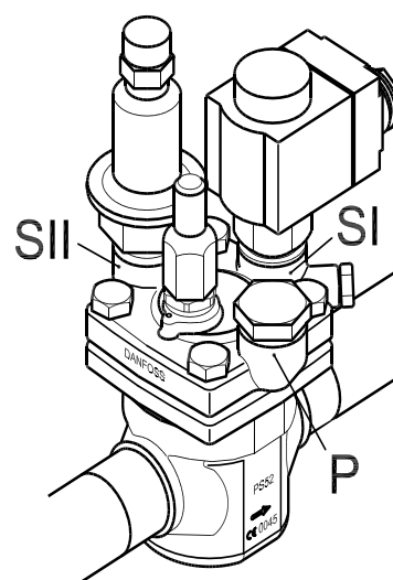
Example (ICS with 3 pilot valves)
