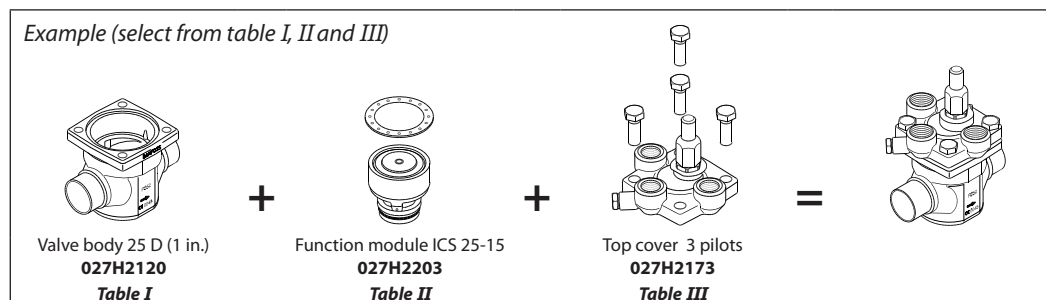
ICV 25 valve body w/different connections Table I
