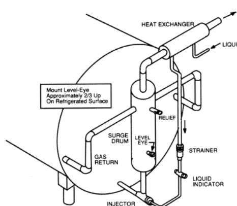
Bulk Tank Ex. (critically charged)
