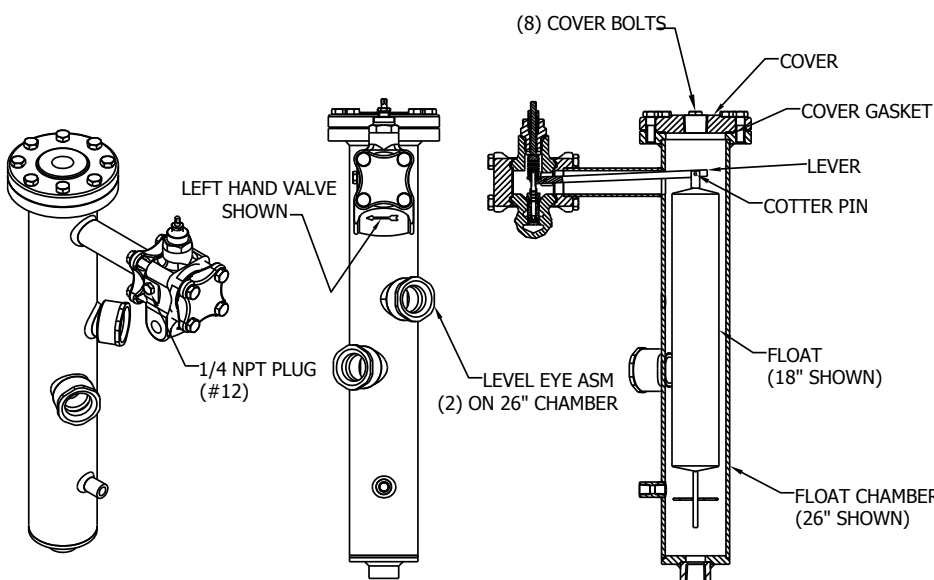
101 Valve Series Assembly with 26" Long Chamber
