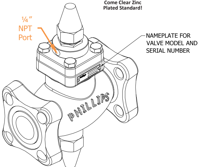
700AP Gas Powered Adjustable Cracking Pressure Check Valve Assembly and Internals
