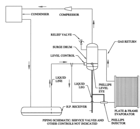
Central Plant System Diagram
