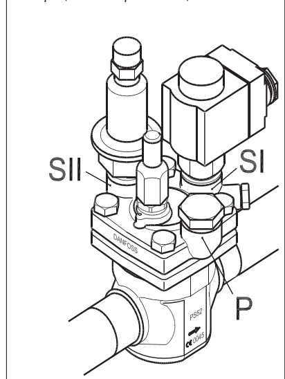
Example (ICS with 3 pilot valves)
