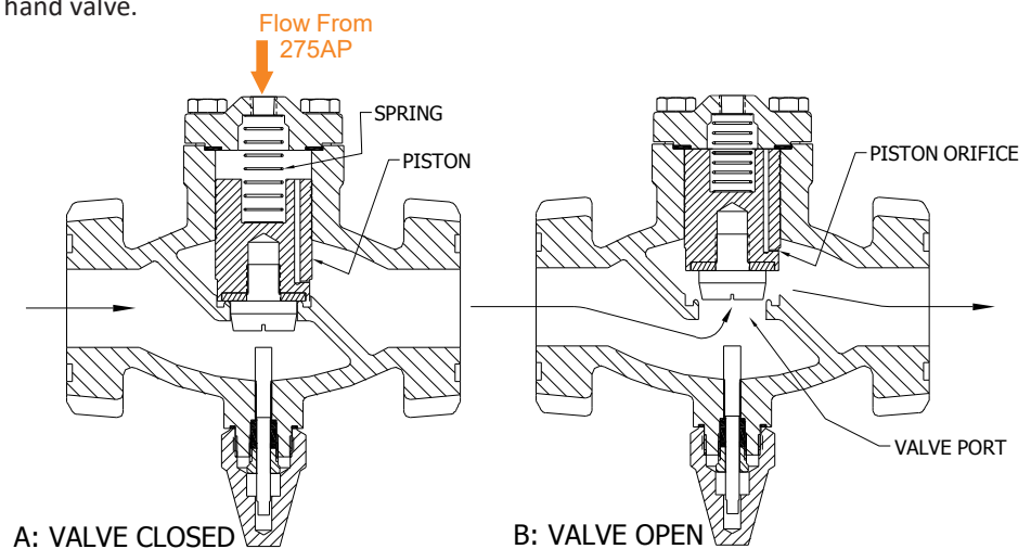
700H Series Operation (valve closed left) (valve open right)
