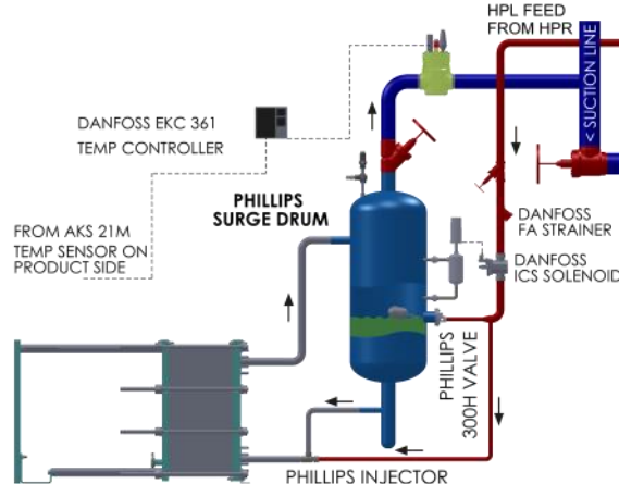
Central Plant System Evaporator Setup
