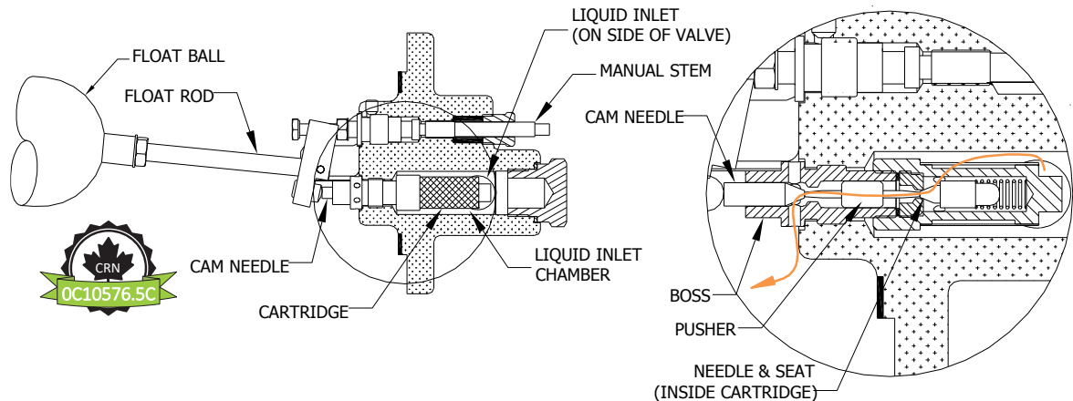
300H Series Design (expands directly through valve into vessel)
