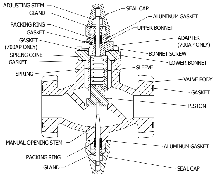
700AP Gas Powered Adjustable Cracking Pressure Check Valve Assembly and Internals
