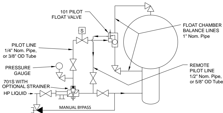
General Application for 701S Series Pilot Operated Valve with 101 Series Adjustable Level Pilot Float Valve
