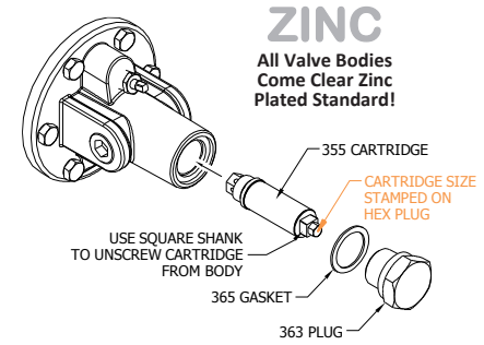
Easily Serviceable Cartridge Design
