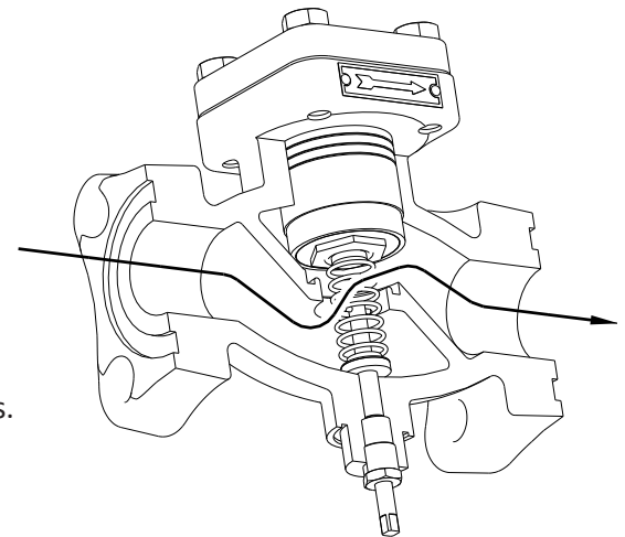
700S Series Permissible Flow Direction
