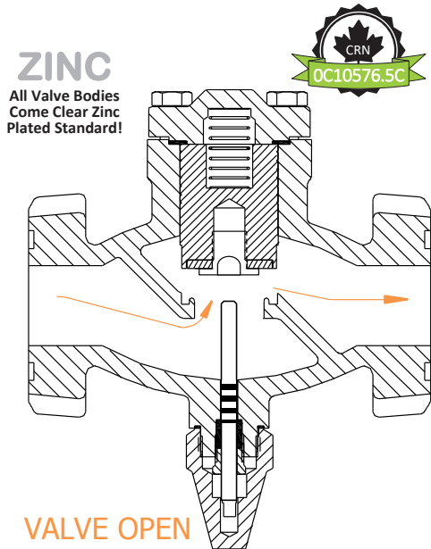
700X Series Piston Type Check
