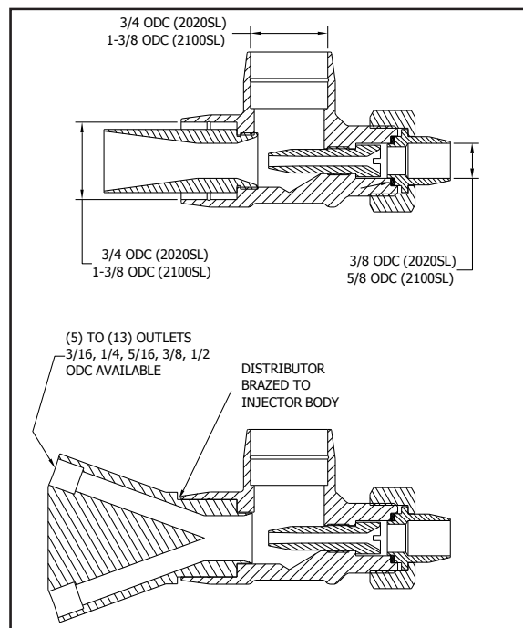
2020SL & 2100SL Injectors
