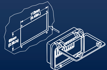
EKE/EKC Panel Kit Mounting Kit w/ Transparent Flip Up Door
