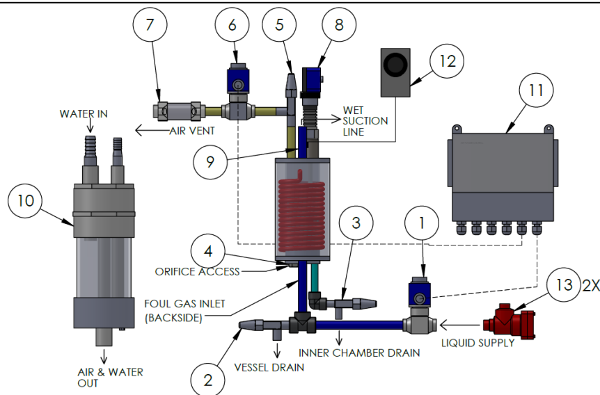
Figure 1: PURJR Air Purger General Layout
