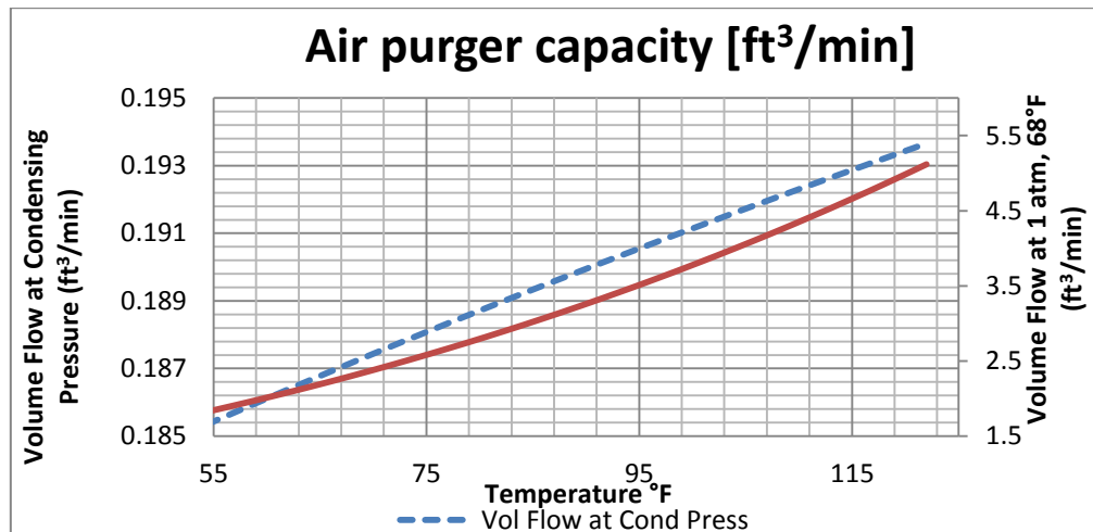
Figure 2: Purger Capacity
