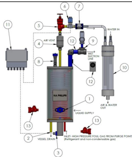
Figure 1: PUR Air Purger General Layout
